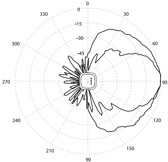
Surveillance range by the radar.
